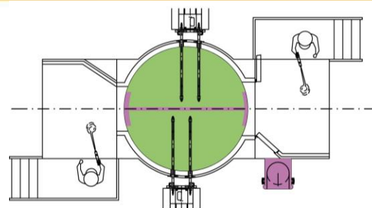
MagicCylinder EquiFlow
